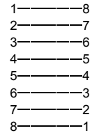
RJ-45 RJ-45
